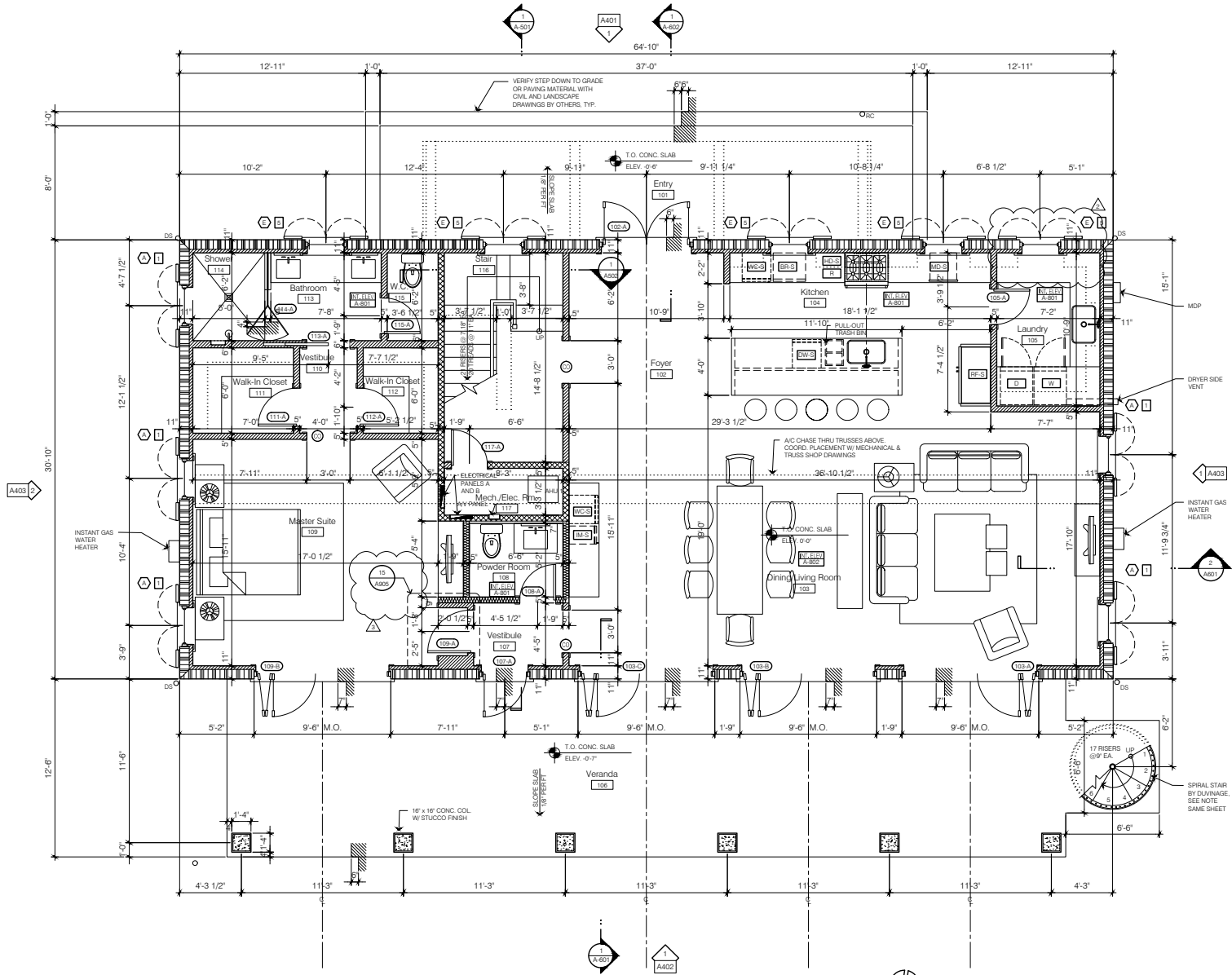
Ground Floor Plan 1/4"
