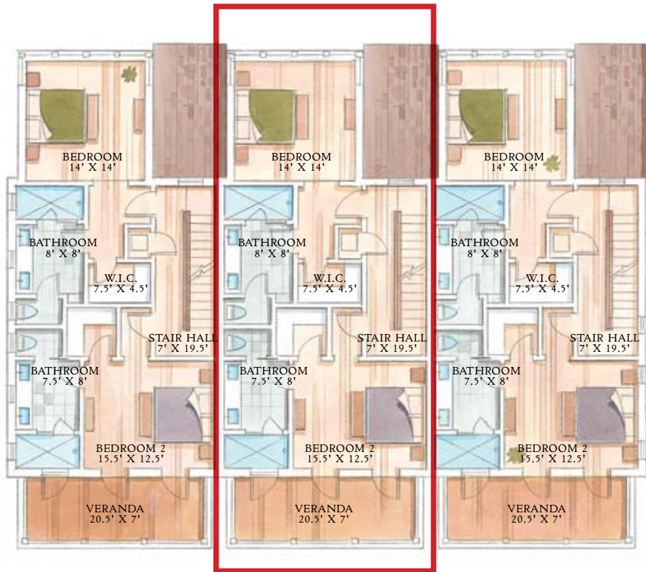
SECOND FLOOR
