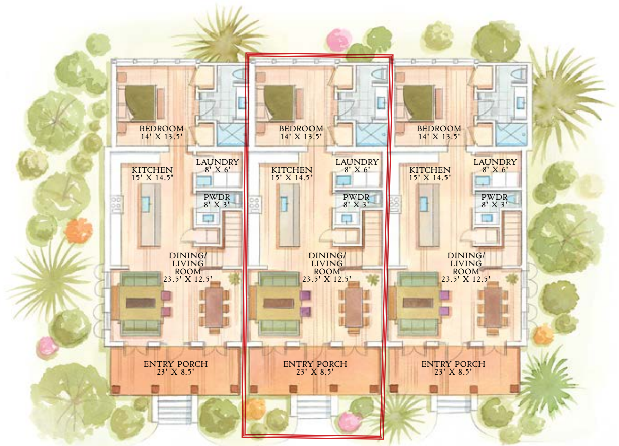
FIRST FLOOR
